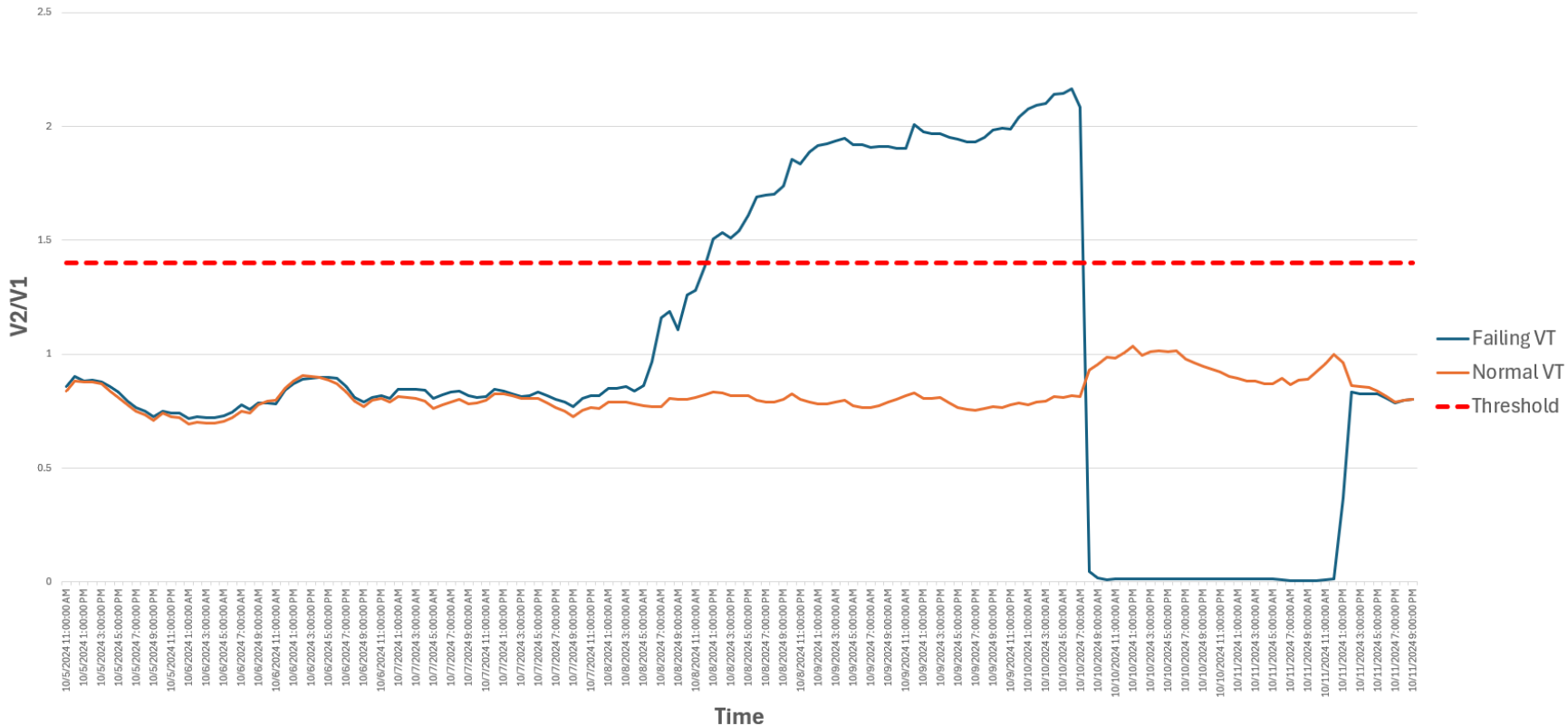
V2/V1 PMU Data For Failing and Normal VT
